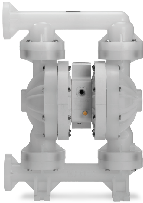
Wilden® 38 mm (1-1/2") Pro-Flo® SHIFT Series Bolted Plastic AODD Pump
