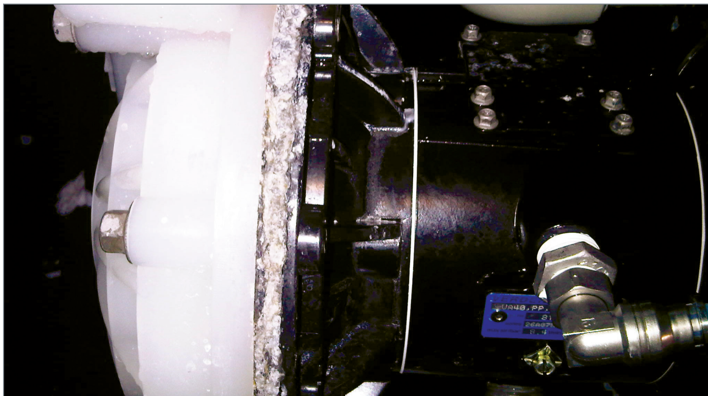
The aluminum materials in this air-operated double-diaphragm (AODD) pump had corroded at the diaphragm, leading to an extremely dangerous situation where workers were at risk of exposure.
