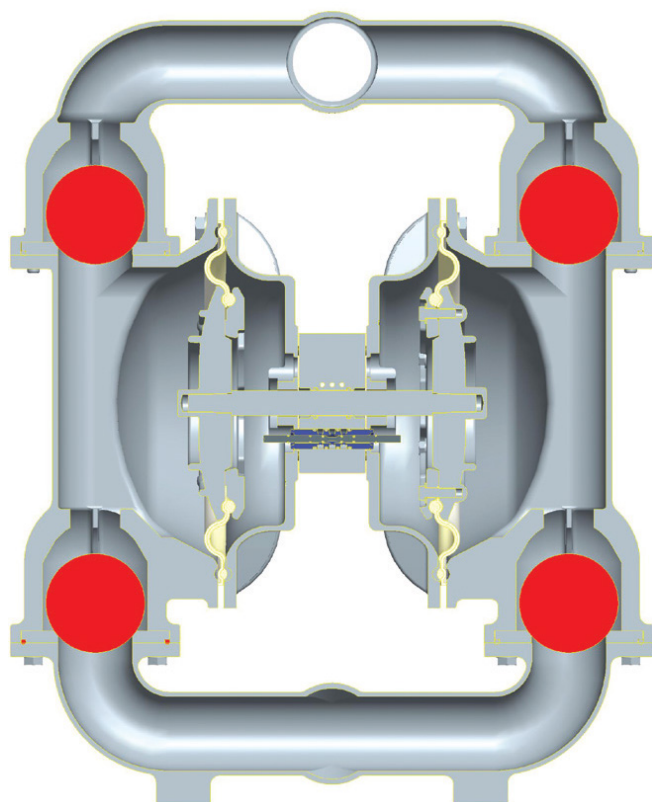
A cross section of the wetted path of the 76 mm (3") Pro-Flo® SHIFT Series Bolted Metal AODD Pump
