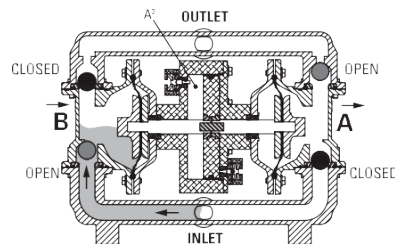
FIGURE 1 When air pressure is supplied to the pump, the air valve directs pressure to the back side of diaphragm (A). The compressed air moves the diaphragm away from the center section of the pump. Simultaneously, compressed air is also supplied to the back side of the power piston (A2); pressure on Area A2 exerts force on the shaft communicated to diaphragm A. This force, when added to the force of pressure A is connected to the process fluid, thus providing the increase of liquid output pressure.
