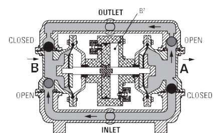
FIGURE 3 At the completion of the stroke, once again the pressure relief valve opens and shifts the air valve. The air valve redirects air to the back side of diaphragm (A) and the power piston (A2), the air behind diaphragm (B) and the power piston (B2) is now exhausted. As the pump reaches its original starting position, each diaphragm has gone through one suction and one discharge stroke of the wetted path and one pressure and exhaust stroke of the air distribution system. This completes one cycle of the high pressure H220.
