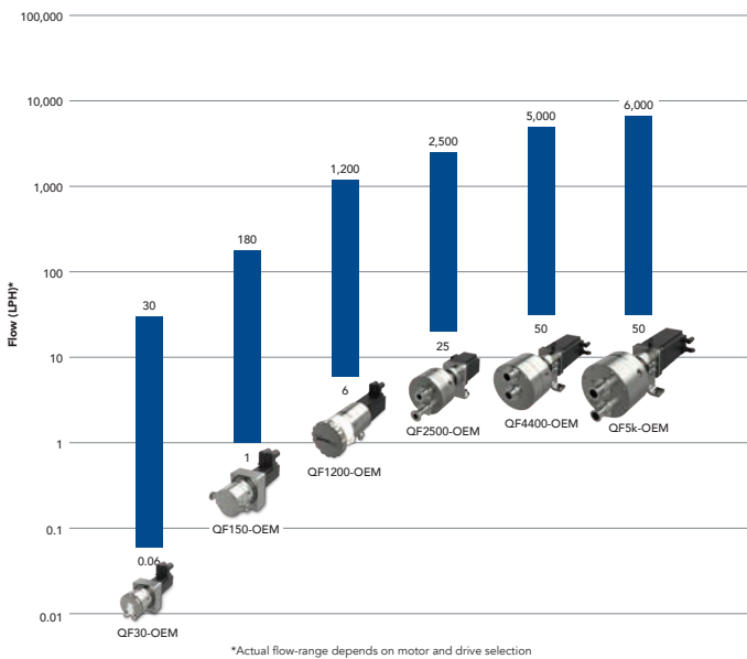
Quattroflow OEM Pump Range
