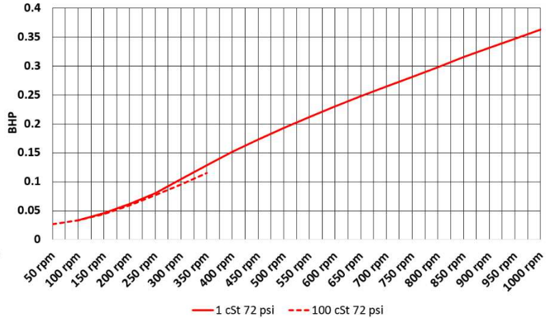
Absorbed power
