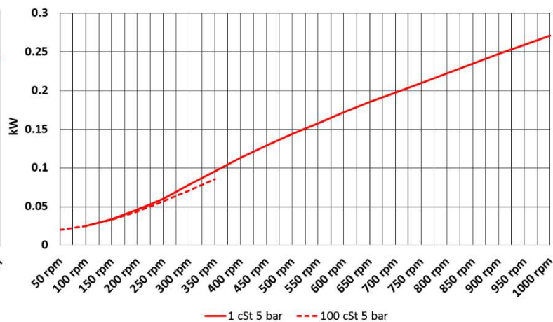
Absorbed power
