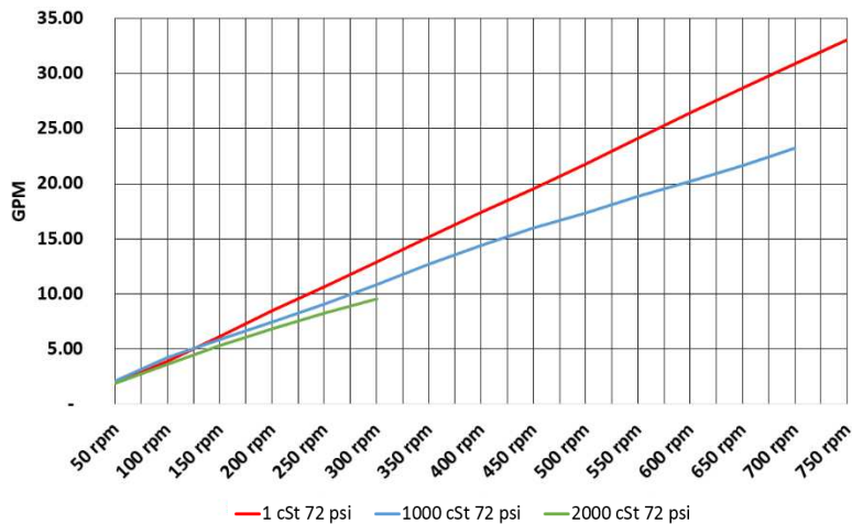
Flow rate vs. RPM
