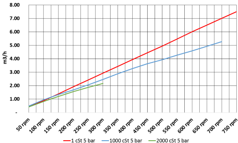
Flow rate vs. RPM
