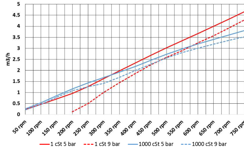
Flow rate vs. RPM
