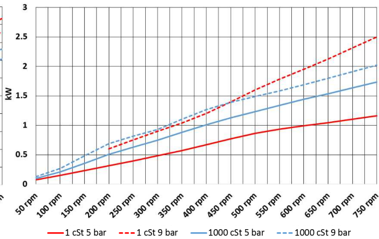
Absorbed power
