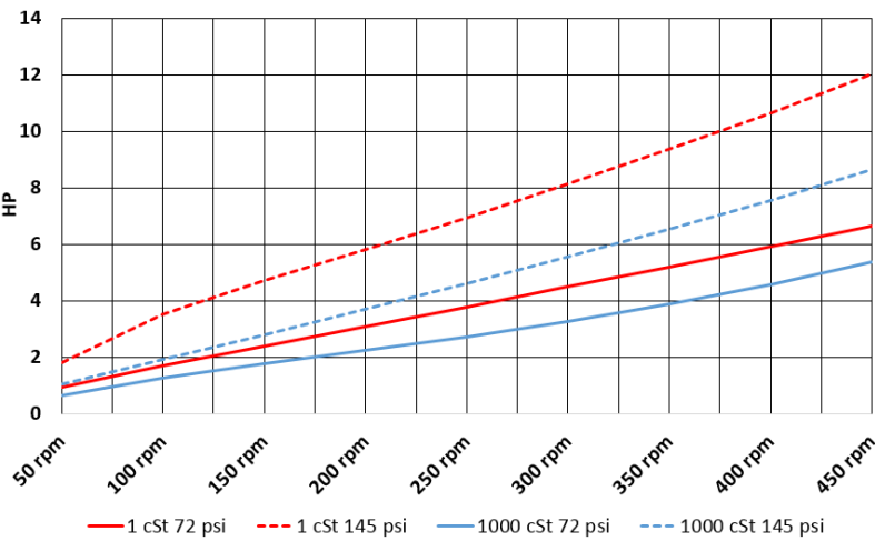
Absorbed power
