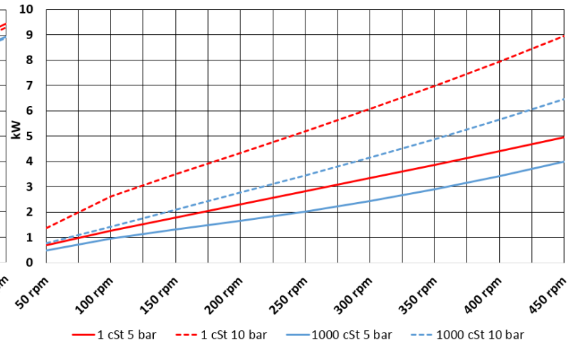
Absorbed power
