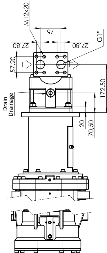
TYPHON II - Hydraulic kit
