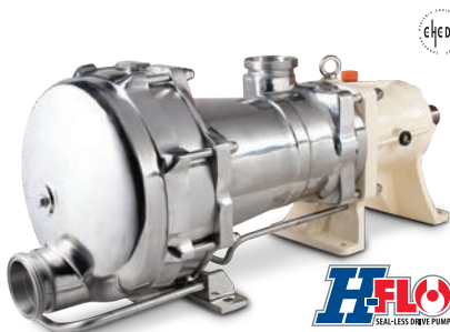
H-FLO Series CIP-capable seal-less pump for various applications. Up to 70 m 3 /h (300 gpm)
