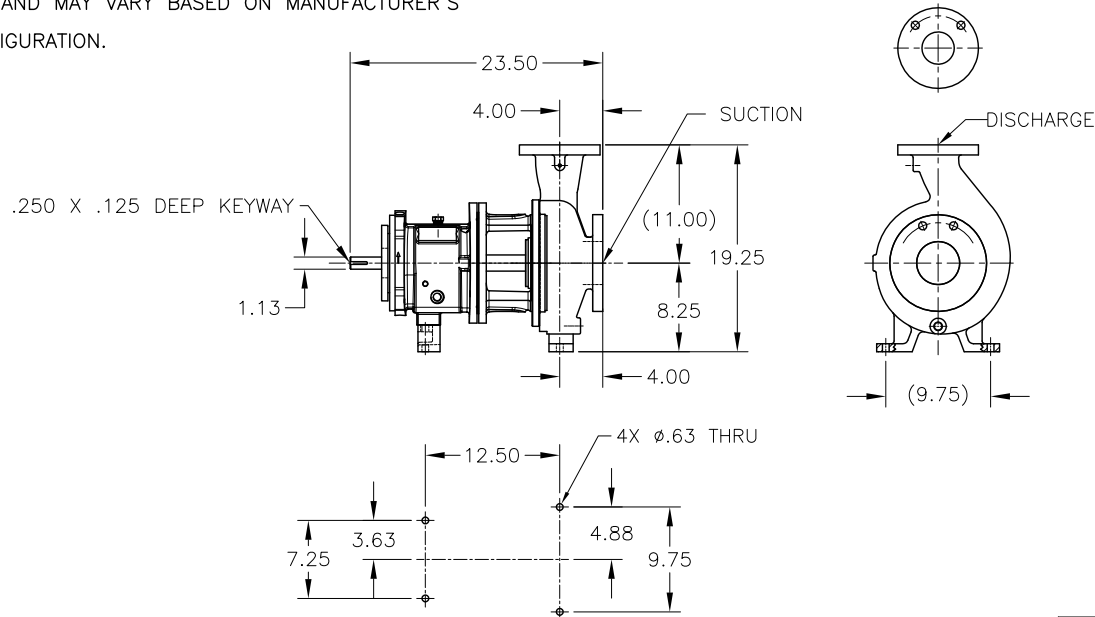
FLANGE OPTION DIMENSIONS
