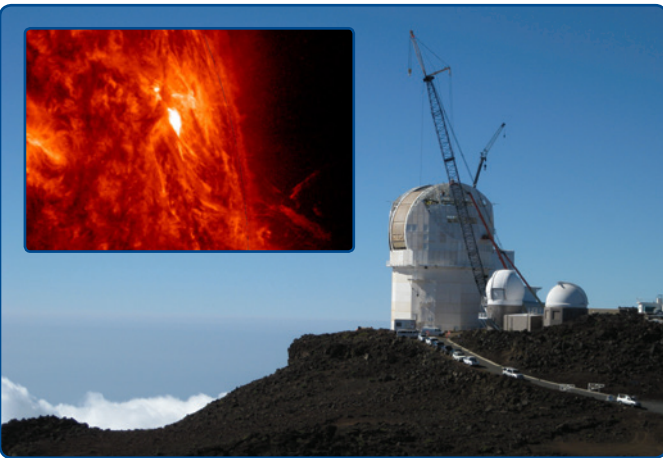
The DKIST will study solar phenomena such as these superheated plasma loops in much greater resolution than possible with current installations. (Courtesy of NASA SDO Instrument Teams).
