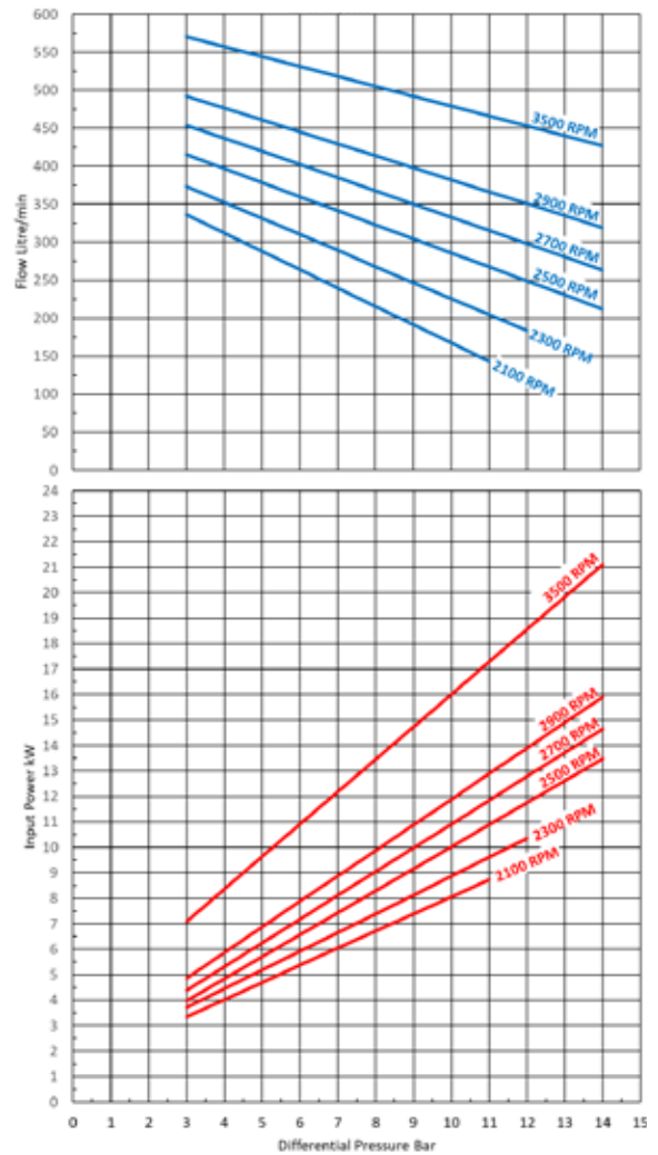
R75 AND R80 PERFORMANCE Liquid: Propane 0.5 S.G.
