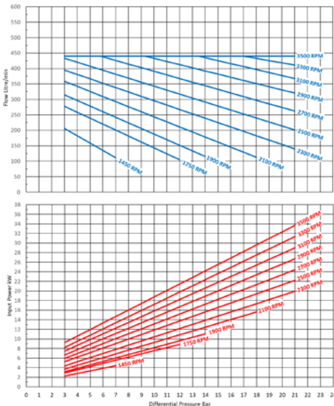
R75 AND R80 PERFORMANCE Liquid: 0.8 S.G. - 5 cSt
