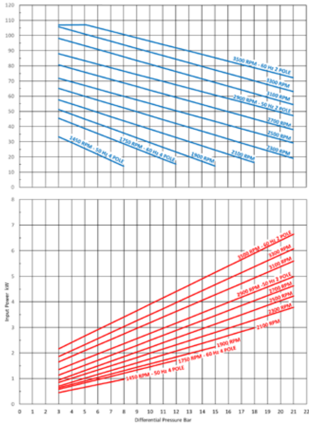
RC25 PERFORMANCE Liquid: 0.8 S.G. - 5 cSt
