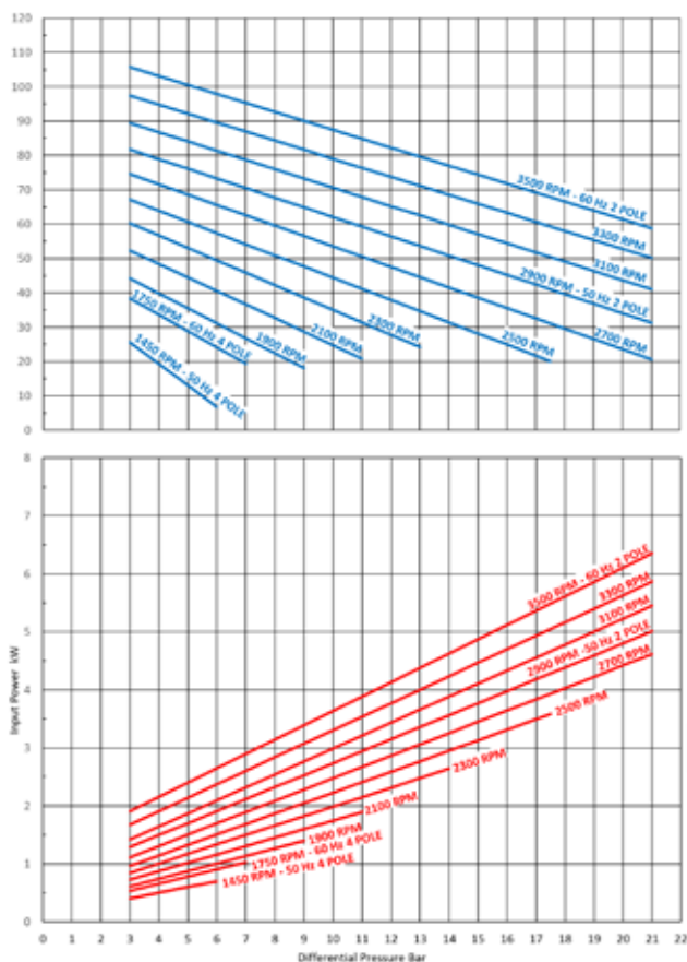
RC25 PERFORMANCE Liquid: 0.8 S.G. - 5 cSt
