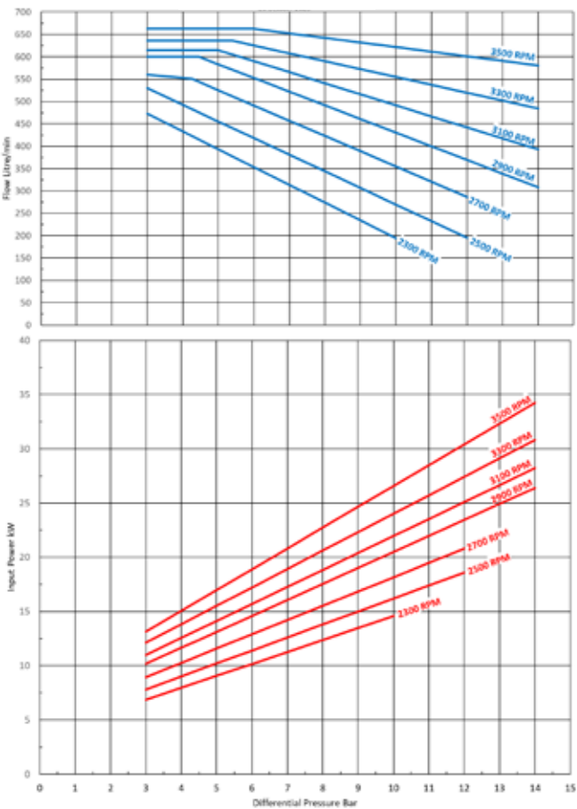
R77 AND R82 PERFORMANCE Liquid: Propane 0.5 S.G.
