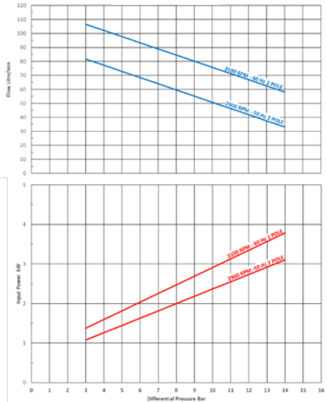
RC25 PERFORMANCE Liquid: Propane 0.5077 S.G.
