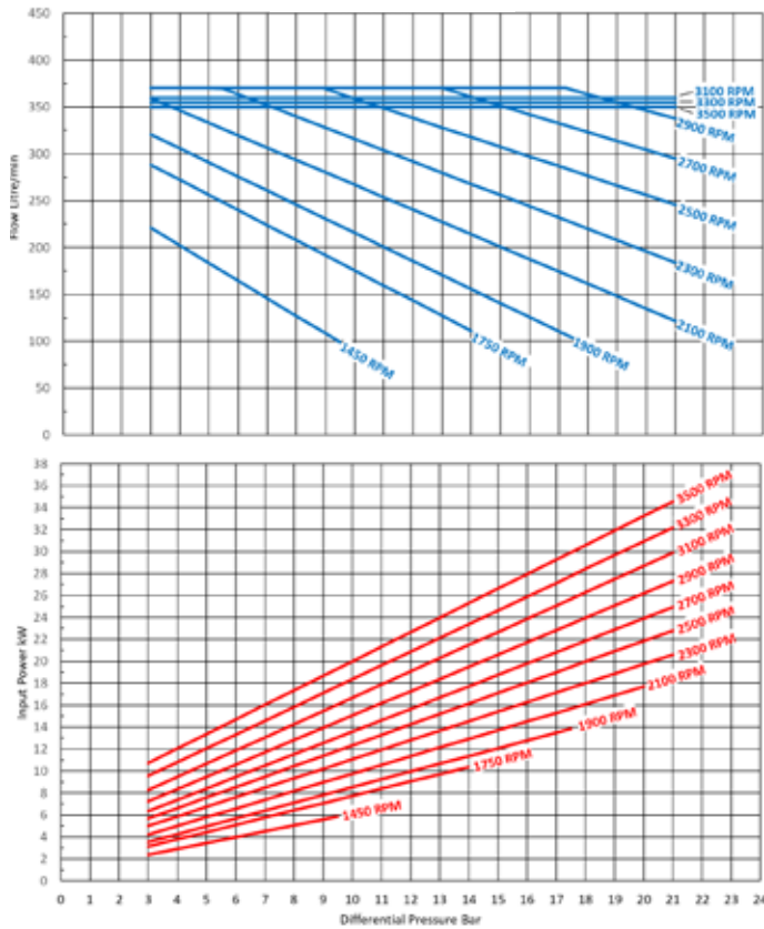
R75 AND R80 PERFORMANCE Liquid: 1.0 S.G. - 1 cSt
