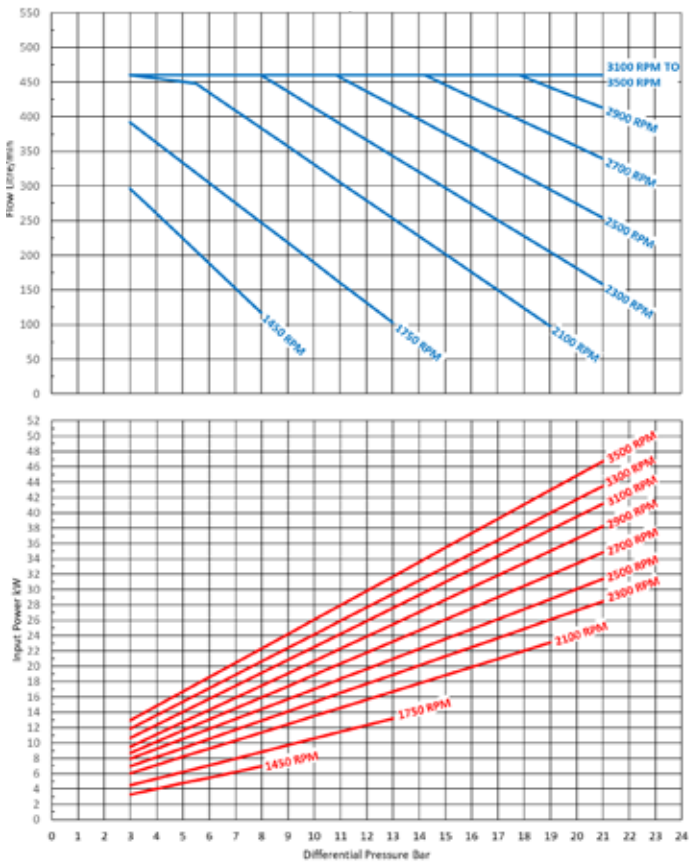
R77 AND R82 PERFORMANCE Liquid: 0.8 S.G. - 5 cSt
