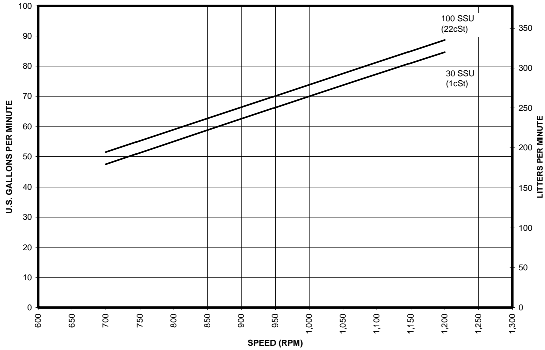
FLOW AT 50 PSI (3.45 Bar)
