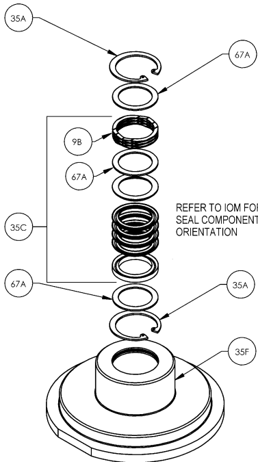
UPPER PACKING ASSEMBLY 1st STAGE
