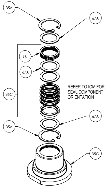
UPPER PACKING ASSEMBLY 2nd STAGE
