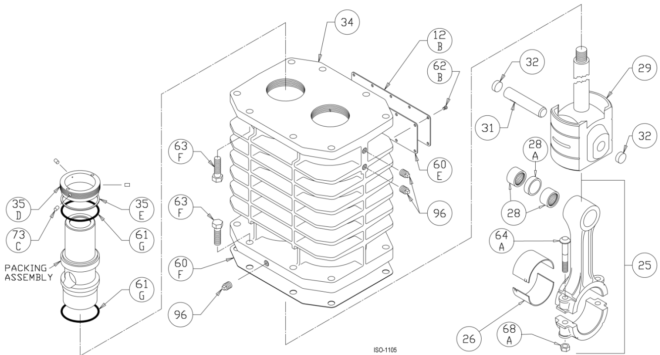
Crosshead Assembly: HD602C, HDL602C, HDL642C, HD612C, HDL612C
