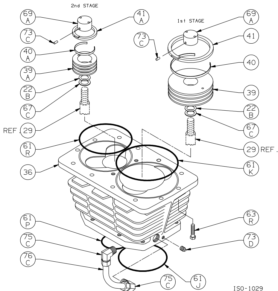
Cylinder Assembly: HD612C|B|A, HD613C|B
