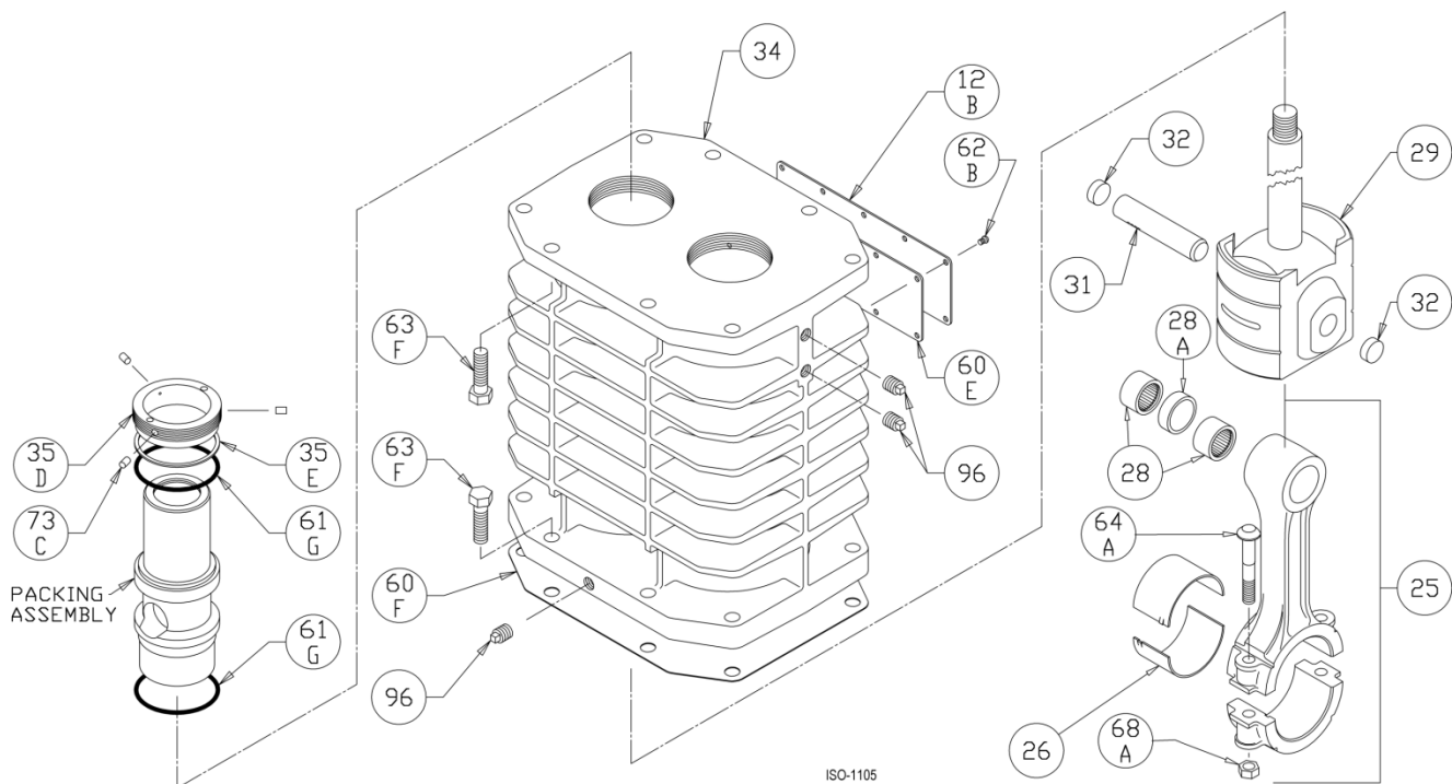
Crosshead Assembly: HD602C, HDL602C, HDL642C, HD612C, HDL612C
