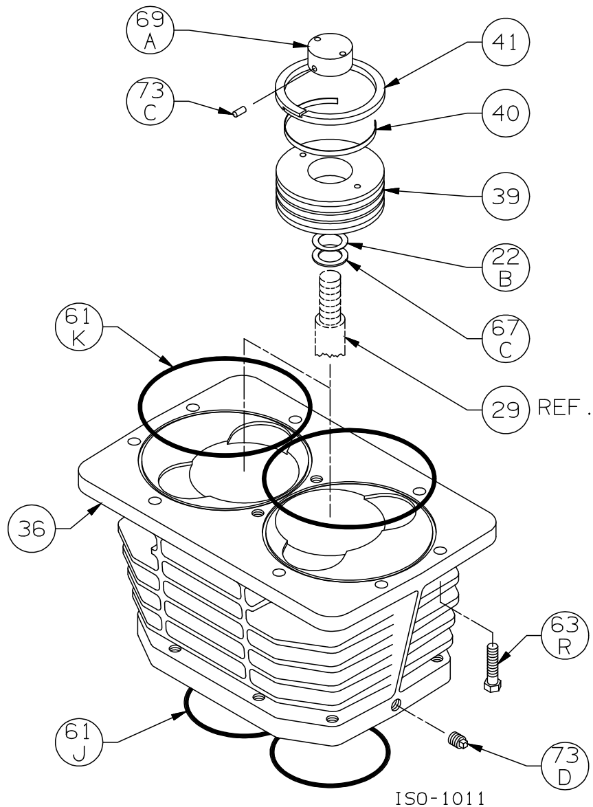
Cylinder Assembly: HD601B|A, HD602C|B|A, HD603C|B|A
