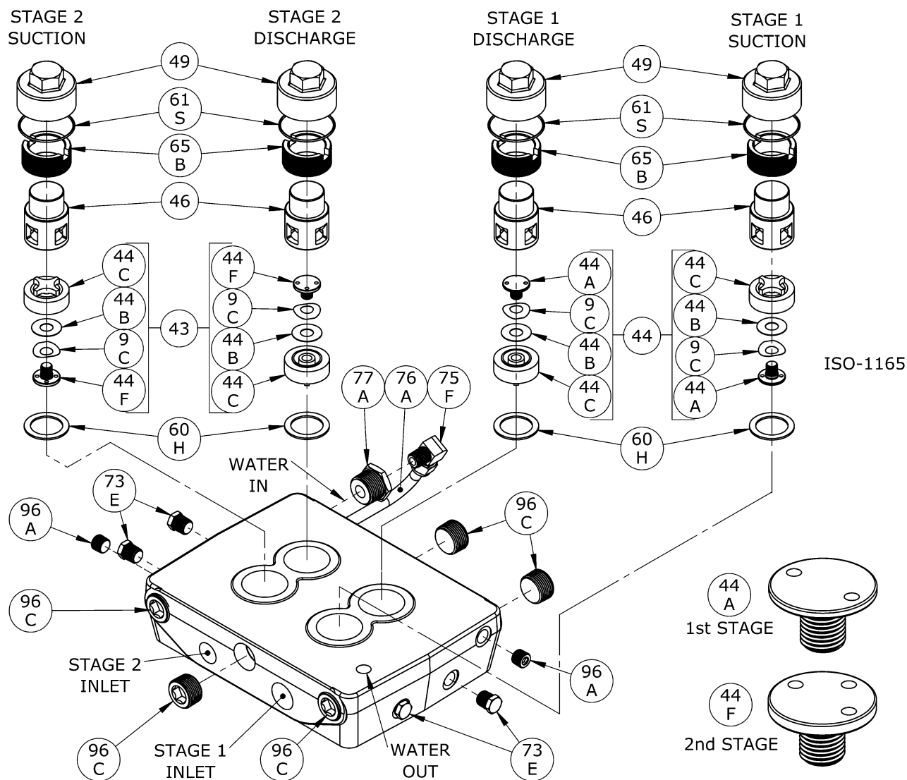
Head Assembly: HDL172C, HDL173C
