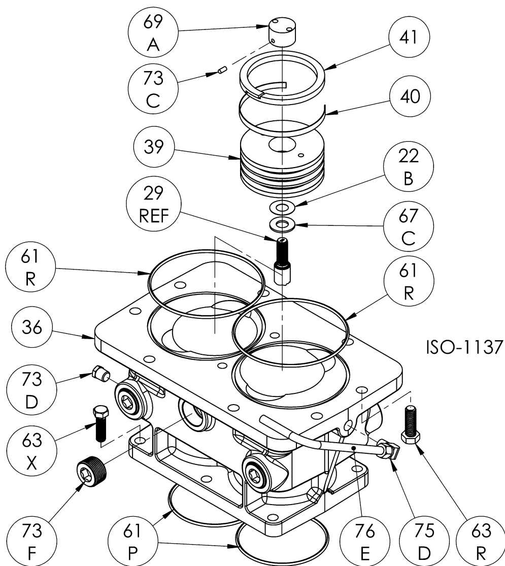
Cylinder Assembly: Models HDL322C, HDL323C
