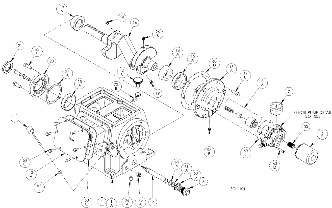
Crankcase ISO1101
