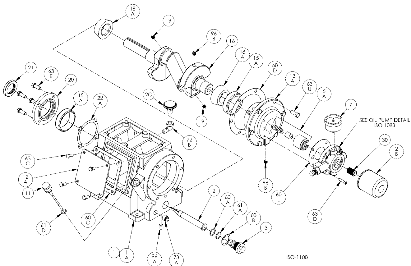
Crankcase ISO1100
