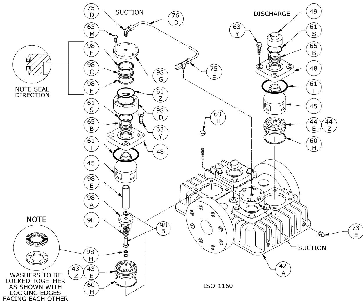
Head Assembly with Unloaders: HD601B|A, HD602C|B|A, HD603C|B|A
