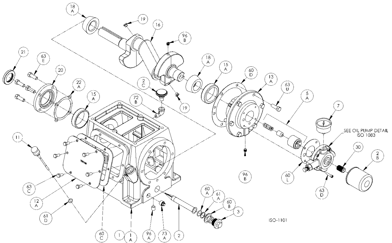
Crankcase ISO1101
