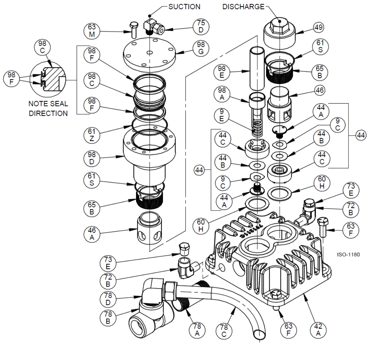
Head Assembly with Unloaders: Model NGS082
