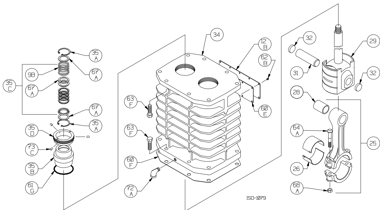
Crosshead Assembly: LB601B
