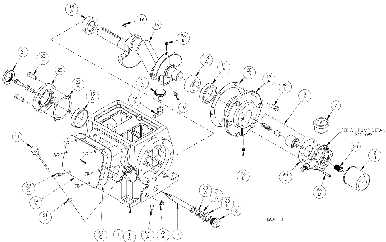
Crankcase Assembly: Models LB361B, LB362D
