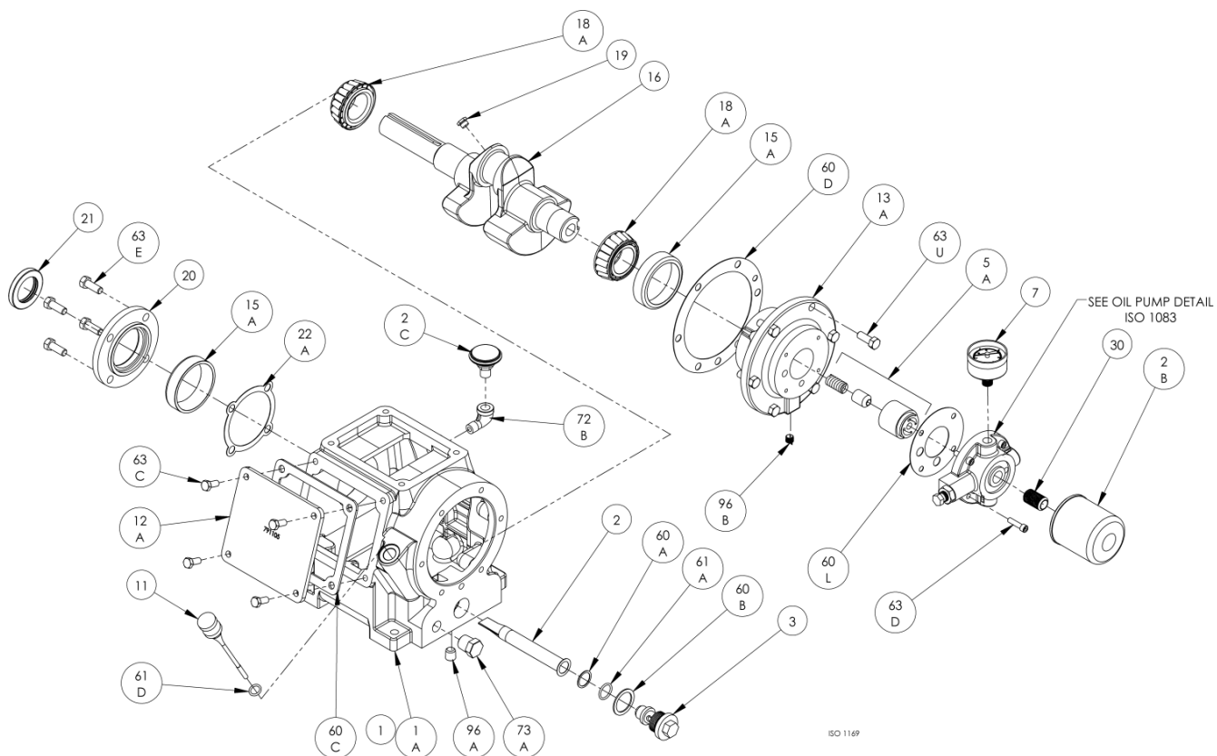
Crankcase Assembly: Model LB082ECA
