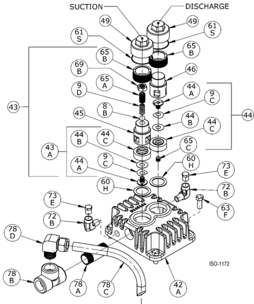
Head Assembly: Model LB082ECA
