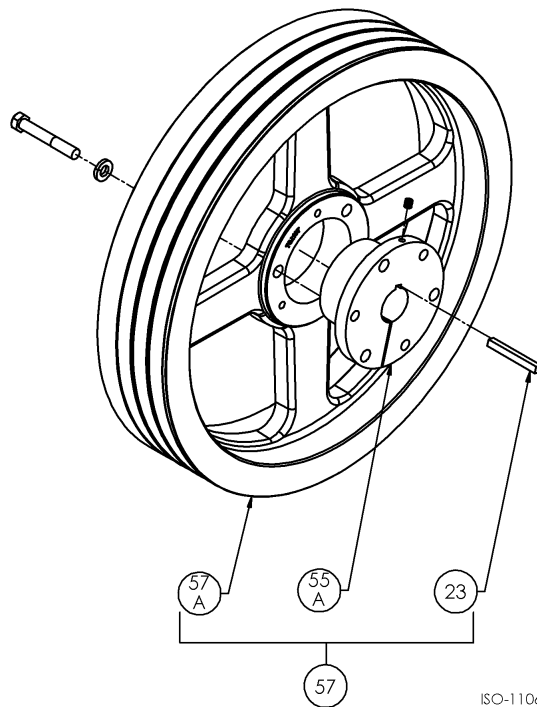
Flywheel Assembly: Model LB082ECA ISO-S1106
