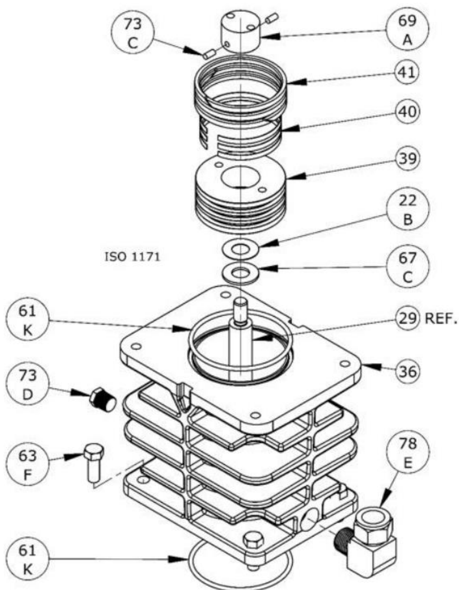
Cylinder Assembly: Model LB081B, LB082B
