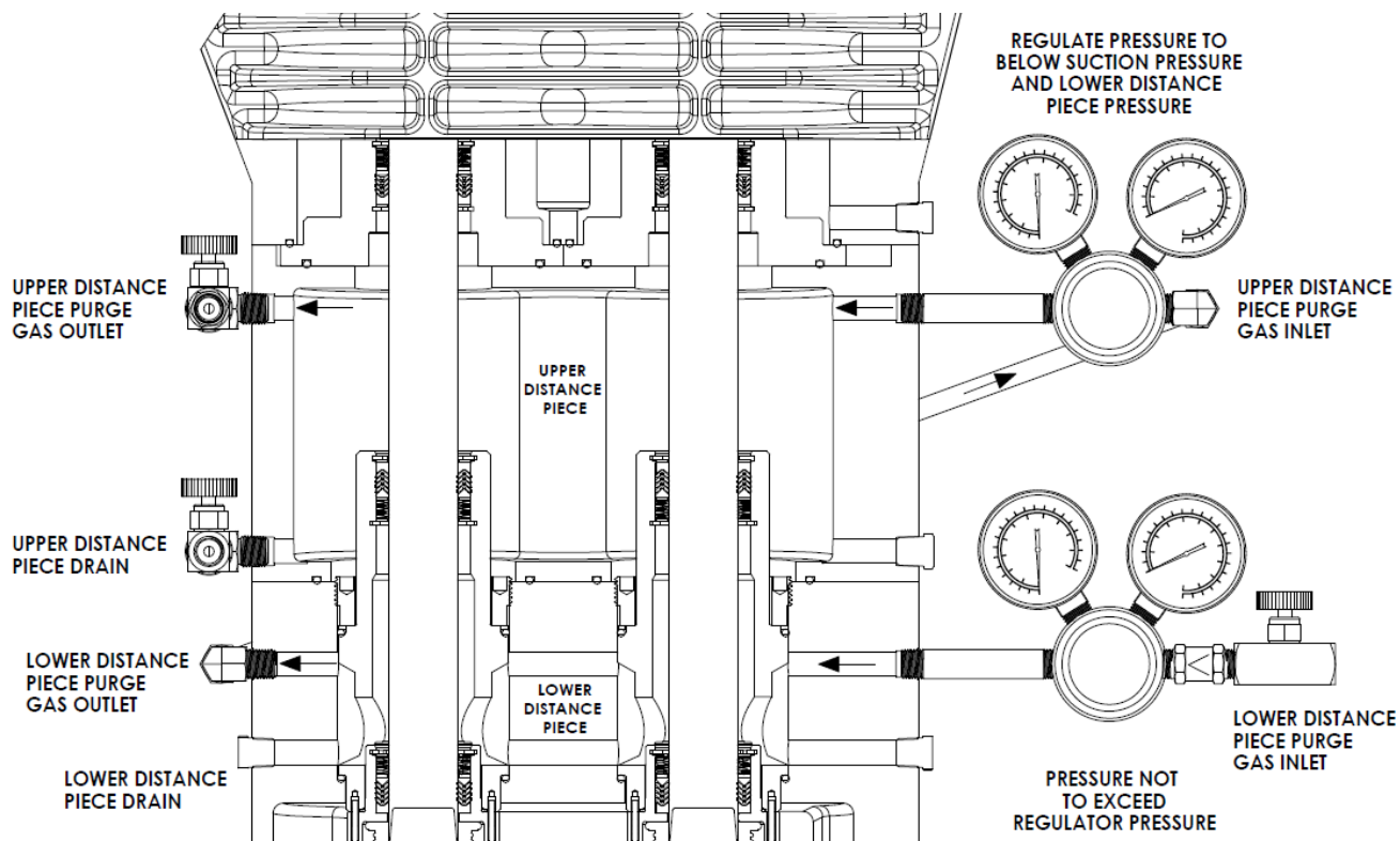
Purge Kit Flow Path – Front View – Typical Triple Seal – Type 5
