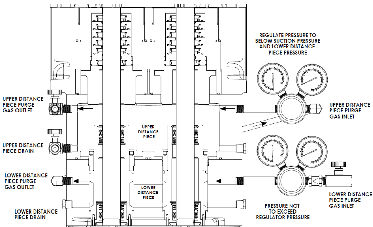
Purge Kit Flow Path – HD943 Triple Seal – Type 5
