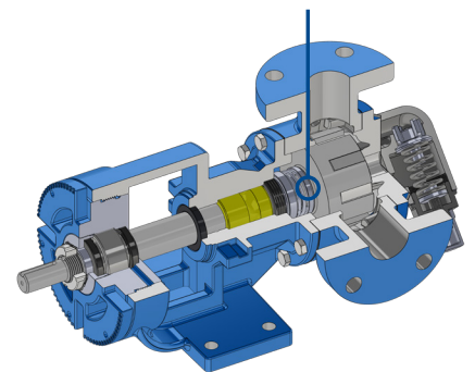
Behind-the-Rotor Seal
