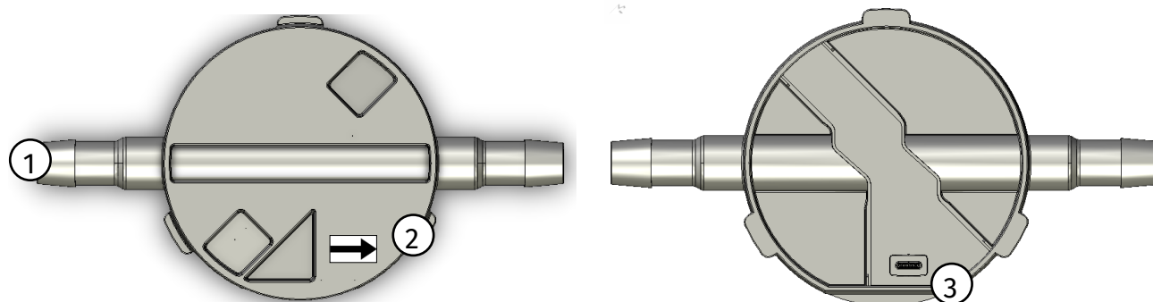
Figure 3: BioProTT™ FlowSU Sensor Description
