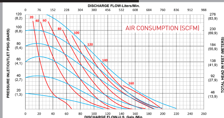
PERFORMANCE CURVE (3" PTFE)*
