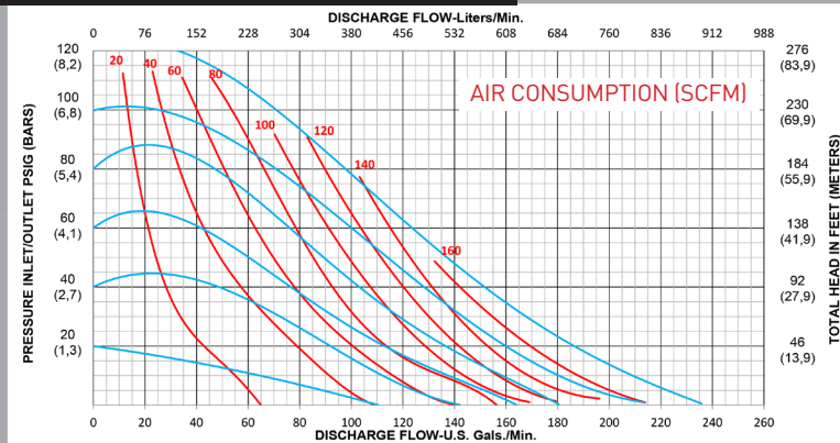
PERFORMANCE CURVE (3" RUBBER)*
