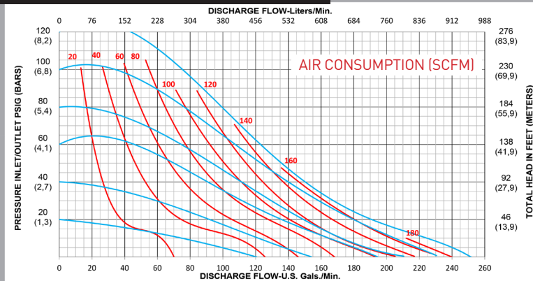
PERFORMANCE CURVE (3" TPE)*
