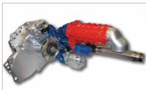
The MH6 from Hydrocar and Mouvex is the world's first combination screw compressor/power take-off unit that is compatible with a truck's gearbox
