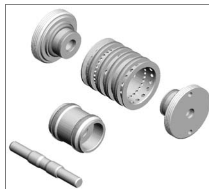
Figure 3 - PERSWING P® - Dismantled
