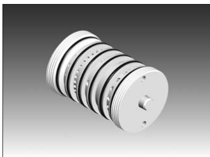
Figure 2 - PERSWING P® Air-Control System
